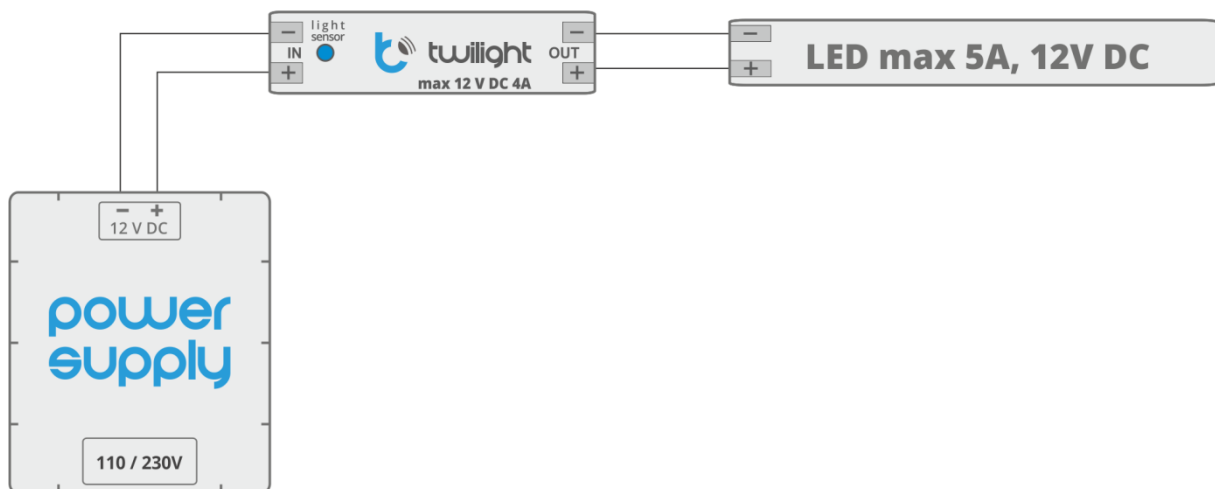
Fig. 2. - Connection diagram
